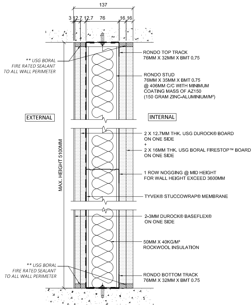
W1 SECTION NTS
